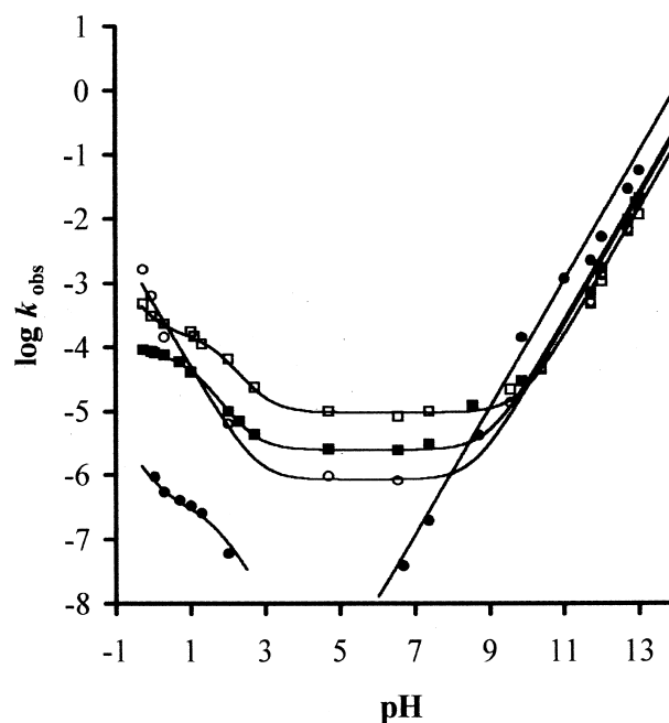
Figure 1. pH-Rate profiles for compounds 7b (●), 7c (■), 7d (□) and 7f (○) at 37°C. Insert: dependence of k_{\text{obs}} with [HCl] for 7f , at 37°C.
