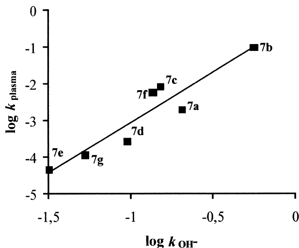
Figure 3. Plot of \log k_{\text{OH}^-} versus \log k_{\text{plasma}} for N -acyloxymethylsulfonamides 7a–g . The data are from Table 3.
