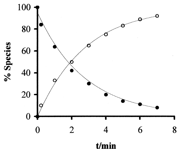
Figure 2. Time-courses for N -benzoyloxymethylnimesulide 7f (●) and nimesulide 5 (○) in the hydrolysis of 7f in 80% human plasma at 37 °C.
