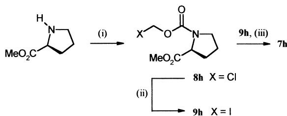
Scheme 1. (i) \text{ClCH}_2\text{OCOC(=O)Cl}/\text{Et}_3\text{N}/\text{CH}_2\text{Cl}_2 ; (ii) \text{NaI}/\text{acetone} ; (iii) 5 (sodium salt)/THF.
